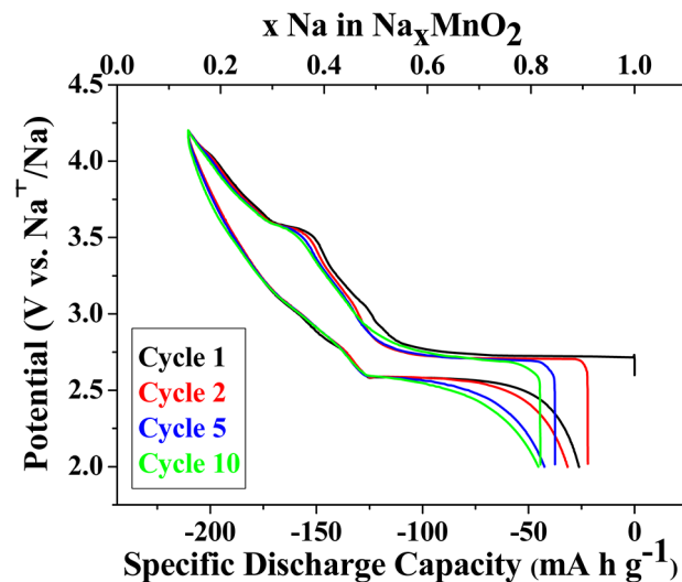
Figure 2. Load curves for \beta - \text{NaMnO}_2 at a rate of C/20 ( 10 \text{ mA g}^{-1} ). The 1st, 2nd, 5th, and 10th Na extraction/reinsertion cycles are represented in black, red, blue and green, respectively.
