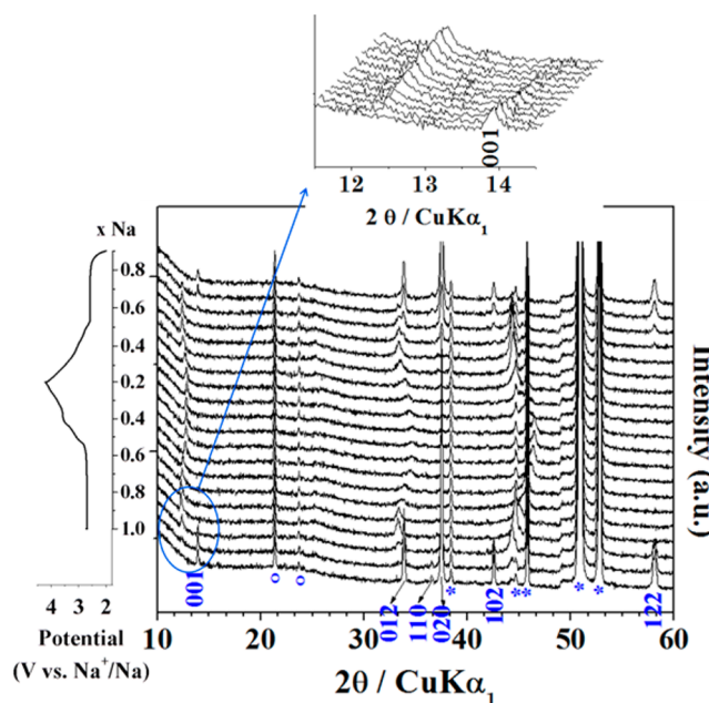
Figure 5. In situ powder X-ray diffraction patterns of \beta - \text{NaMnO}_2 recorded during the first electrochemical cycle at C/10 every 0.08 \text{ Na}^+ exchanged. The region between 12 and 15° in 2\theta is highlighted in order to show the gradual reduction in intensity of the (001) peak, and the gradual appearance of a peak at lower 2\theta angles associated with the two phase deintercalation. The asterisk symbol (*) represents the Be window and the o symbol comes from other components of the in situ cell.
