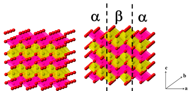
Figure 1. (a) Schematic representation of \beta - \text{NaMnO}_2 in the Pmnm space group and (b) intergrowth model between \alpha and \beta - \text{NaMnO}_2 . \text{MnO}_6 octahedra are pink, \text{NaO}_6 octahedra are yellow, and O atoms are red. Adapted from Abakumov et al. 36 copyright 2014 American Chemical Society.
